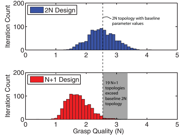
Fig. 8. Histogram of grasp quality values from Monte Carlo simulations for two-finger grasp, 2N and N+1 designs. The N+1 topologies exceeding the baseline 2N topology are shaded gray.
