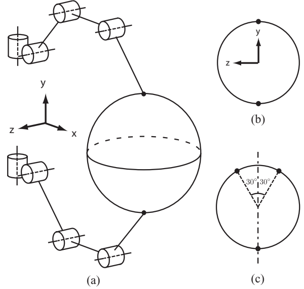
Fig. 6. Grasp configurations analyzed. (a) Isometric view of two-finger grasp. (b) Front view of two-finger grasp. (c) Side view of three-finger grasp.
