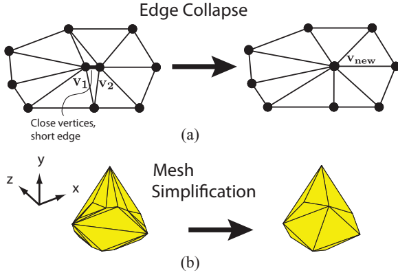
Fig. 4. (a) Example of an edge collapse operation. The vertices v_1 and v_2 are collapsed into a new vertex v_{new} . Adapted from [35]. (b) Example of using edge collapse operations to simplify the feasible object force set from 19 vertices down to 10 vertices. Note that this view is of the underside of the feasible object force set in Fig. 3.
