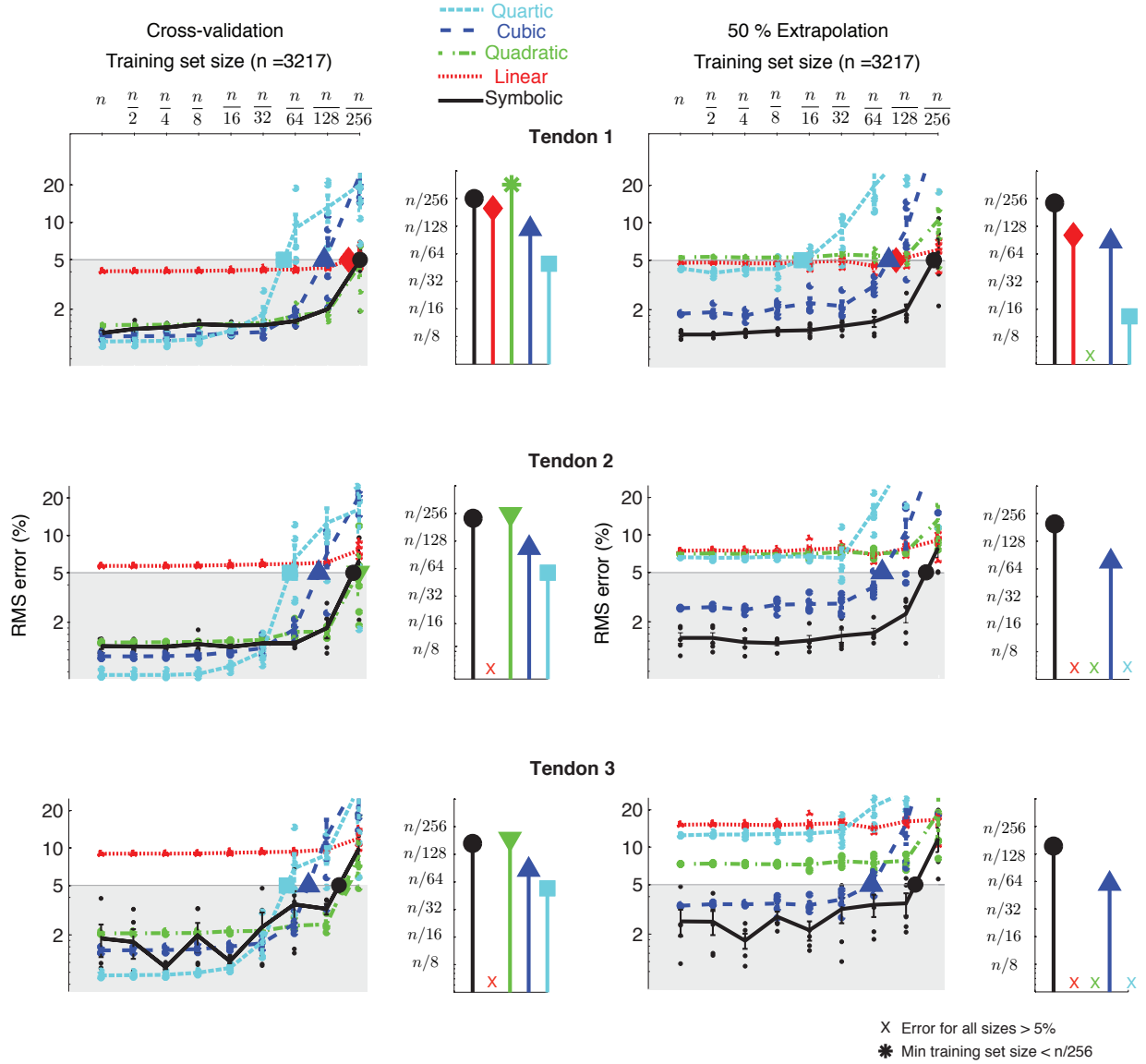
Fig. 3. Effect of reducing the size of the training dataset : Comparison of RMS errors of symbolic and polynomial regressions with reduction in the number of training data points. The plots show mean and standard errors calculated across five runs for each regression type and training dataset size for the three tendons of the experimental robotic finger. When tested with the cross-validation dataset (interpolated from the same range as the training dataset), cubic and quartic regression had lower RMS errors compared to symbolic regression for large training datasets and quadratic regression had errors comparable to symbolic regression for small training datasets. But when tested with the extrapolation dataset (data points outside the range of training upto 50% of the volume of the training dataset), symbolic regression had lower errors than all polynomial regressions for all the different training dataset sizes. The stem plots show the training dataset size required to obtain a 5% RMS error using each of the regression techniques. Symbolic regression requires the fewest training data points compared to the different polynomial regressions for 5% cross-validation and extrapolation errors.
