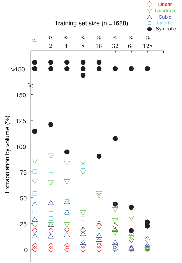
Fig. 5. Summary of the comparison between symbolic and polynomial regressions in their ability to extrapolate and their performance with training dataset reduction. The achievable percentage extrapolation for models trained over different training dataset sizes to maintain RMS errors below 5% is shown for each regression technique for the three tendons of the planar robotic system. For each training dataset size, symbolic regression can extrapolate to larger ranges beyond the training dataset compared to polynomial regressions.
