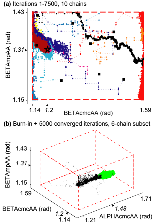
Fig. 6. (a) The overdispersed initial conditions (solid squares) for ten independent Markov chains are shown for two representative parameters for the 36D test case 6. Some chains (e.g., dark red) located the true posterior (true parameter values marked by a star) while others (e.g., black) found local minima. (b) The history of the six-chain subset is shown for three representative parameters for the 36D test case 6. Burn-in and pooled converged iterations are shown in black and green, respectively. For both Subplots a and b , prior distribution bounds are represented by dashed red lines, and tick marks and triangles on the axes indicate the parameter bounds and true values, respectively.
