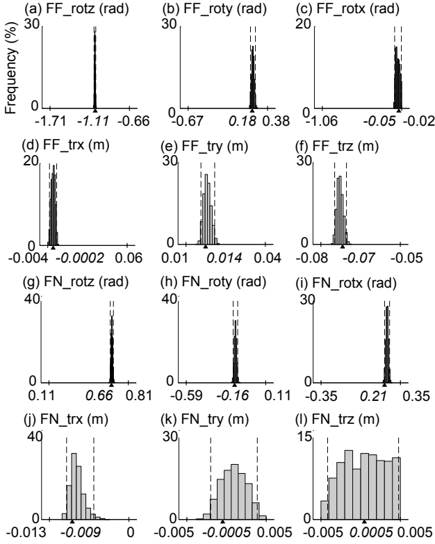
Fig. 9. Marginal distributions are shown for the 12 parameters for the frame transformations at the proximal base and distal tip of the thumb [31] for the 36D test case 6. Dashed lines indicate the 95% confidence intervals while tick marks and triangles on the x-axes indicate the parameter bounds and true values, respectively.
